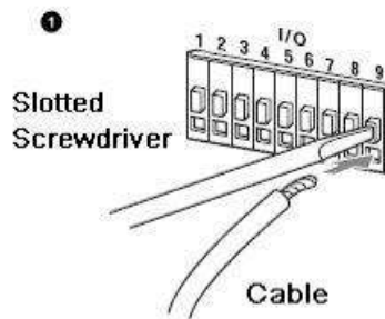
Figure 9-4 Install cable
