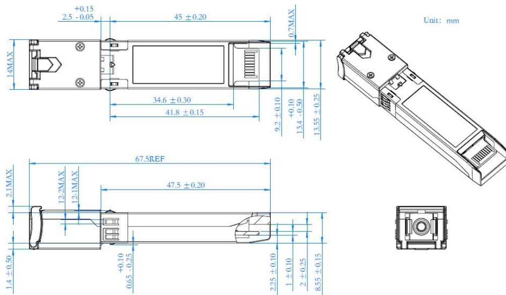
Figure 4 Package Outline
