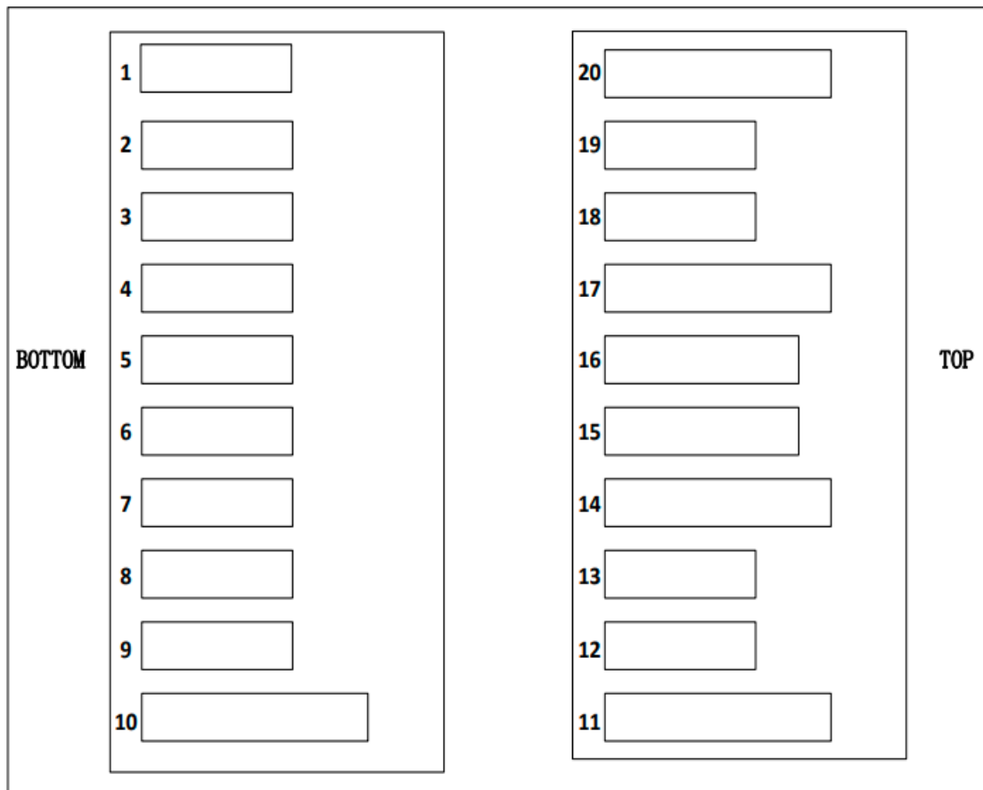
Figure 4 Pin Out Drawing
