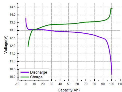
12.8V100Ah Charge-Discharge Curve 0.2C, 25°C
