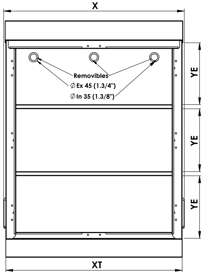
Vista frontal
