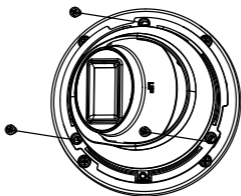
Figure 2-6 Install the Camera to Junction Box's Cover
