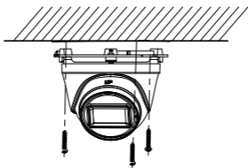
Figure 2-2 Fix the Camera
