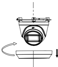
Figure 2-1 Take off the Fixing Ring
