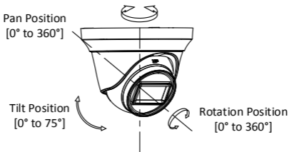
Figure 2-4 3-Axis Adjustment
