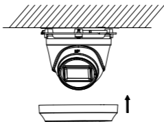
Figure 2-3 Put the Fixing Ring Back
