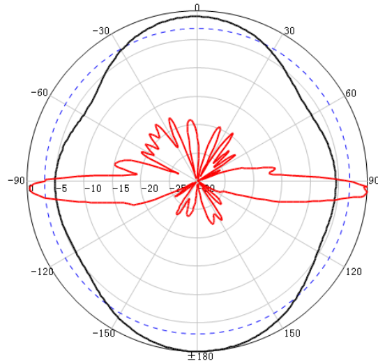
V-Pol @ 2450MHz
