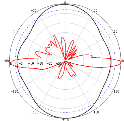
V-Pol @ 2450MHz
